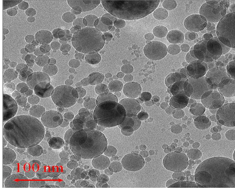
Figure 1.2. TEM image of Al 2 O 3 /water nanofluid - 0.06% vol. concentration (Sommers, 2012).
